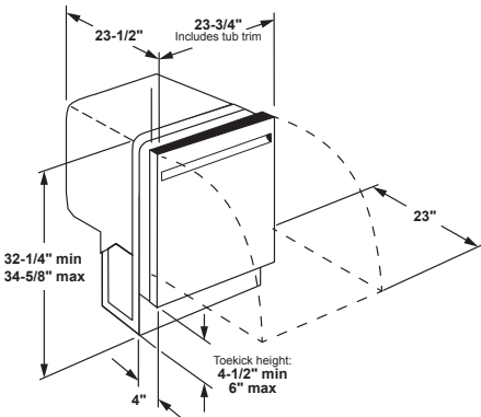
Overall depth including handle: 25.6".
