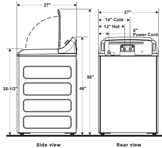
WASHER DIMENSIONS FOR 4.8/4.6 CU. FT. CAPACITY WITH GLASS LID
