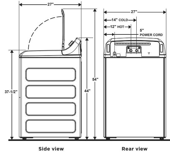
WASHER DIMENSIONS FOR 4.6, 4.5, 4.4, 4.2, 3.8 CU. FT. CAPACITY WITH METAL LID
