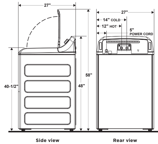
WASHER DIMENSIONS FOR 5.2/5.0 CU. FT. CAPACITY
