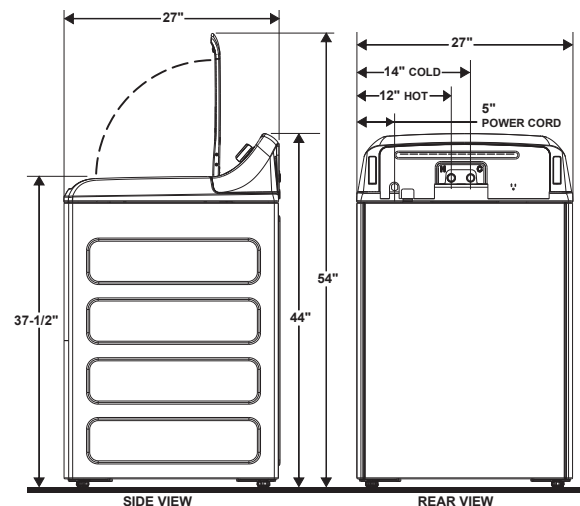
Washer dimensions (inches)
