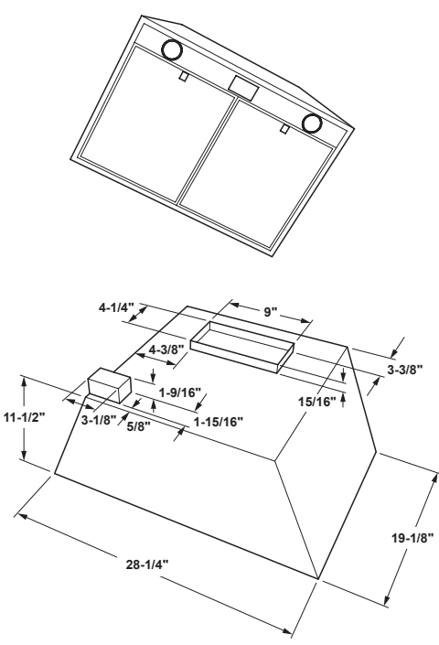
MODEL UVW8364
