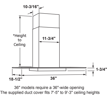
MODEL CVW7361
