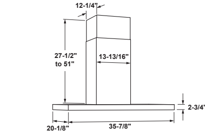
MODEL UVW9361
