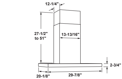
MODEL UVW9301
