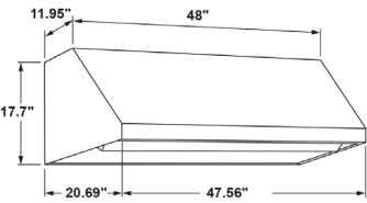
MODEL UVW9484
