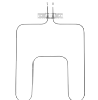
WB44X200 (Installer Pkg) Range Oven Bake Element • Available in 25 pack (WB44X6200) • 3,000 Watts • 240 Volts
