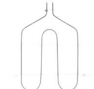
WB44T10009 (Installer Pkg) Range Oven Broil Element • 3,400 Watts • 240 Volts • Available in 25 pack (WB44X6185)
