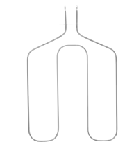
WB44X173 (Installer Pkg) Range Oven Broil Element • 3,400/2,500 Watts • 240/208 Volts
