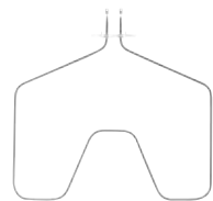
WB44X5082 (Installer Pkg) Range Oven Bake Element • Available in 25 pack (WB44X6082) • Easy to install—contains two screw-on terminals • Designed to fit many different GE ovens; be sure to search by your appliance model number to ensure this part will fit your range • 18-1/4" W X 14-1/4" D to mounting flange; 2,500/1,900 Watts 240/208 volts
