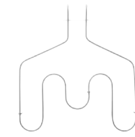
WB44T10011 (Installer Pkg) Range Oven Bake Element • 3,400 Watts • 240 Volts
