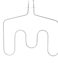
WB44X10016 (Installer Pkg) Range Oven Bake Element • 3,400/2,500 Watts • 240/208 Volts
