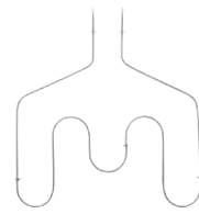
WB44T10011 (Installer Pkg) Range Oven Bake Element • 3,400 Watts • 240 Volts
