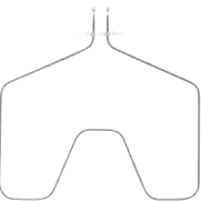
WB44X5082 (Installer Pkg) Range Oven Bake Element • Available in 25 pack (WB44X6082) • Easy to install—contains two screw-on terminals • Designed to fit many different GE ovens; be sure to search by your appliance model number to ensure this part will fit your range • 18-1/4" W X 14-1/4" D to mounting flange; 2,500/1,900 Watts 240/208 volts
