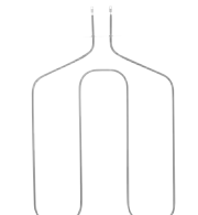
WB44X173 (Installer Pkg) Range Oven Broil Element • 3,400/2,500 Watts • 240/208 Volts
