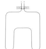
WB44X200 (Installer Pkg) Range Oven Bake Element • Available in 25 pack (WB44X6200) • 3,000 Watts • 240 Volts
